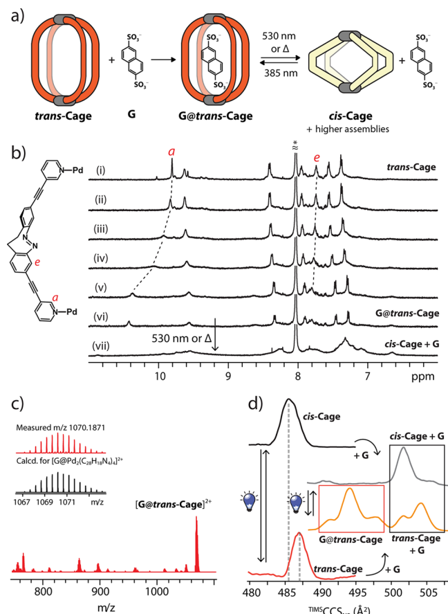
Figure 5. (a) Guest uptake of trans -Cage and release by isomerization to cis -Cage; (b) 1 H NMR (500 MHz, DMF- d 7 , 298 K) stepwise addition of guest G to trans -Cage (mole ratio of host:guest = (i) 1:0.2, (ii) 1:0.4, (iii) 1:0.6, (iv) 1:0.8, and (v) 1:1.0) followed by photoswitching (vii); (c) ESI-MS of G @ trans -Cage; (d) ion mobility spectra for cis -Cage, cis -Cage+ G , trans -Cage, and G @ trans -Cage and light-induced reversibility of the process. The red box highlights signals for inside binding; the black box, signals for outside binding.
